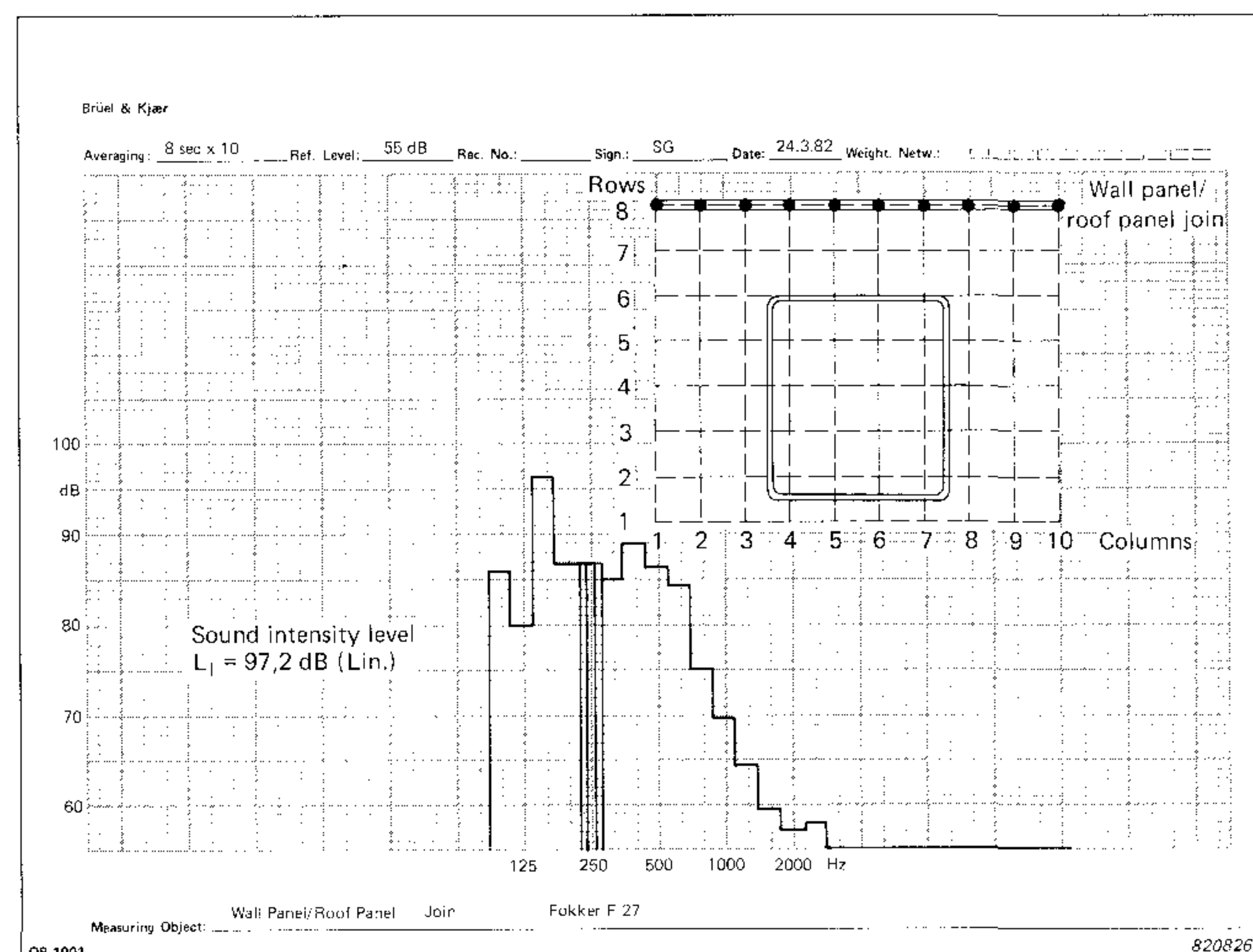
Fig. 7. Sound intensity level over the wall-panel / roof-panel joint area, averaged over 10 measurement points
