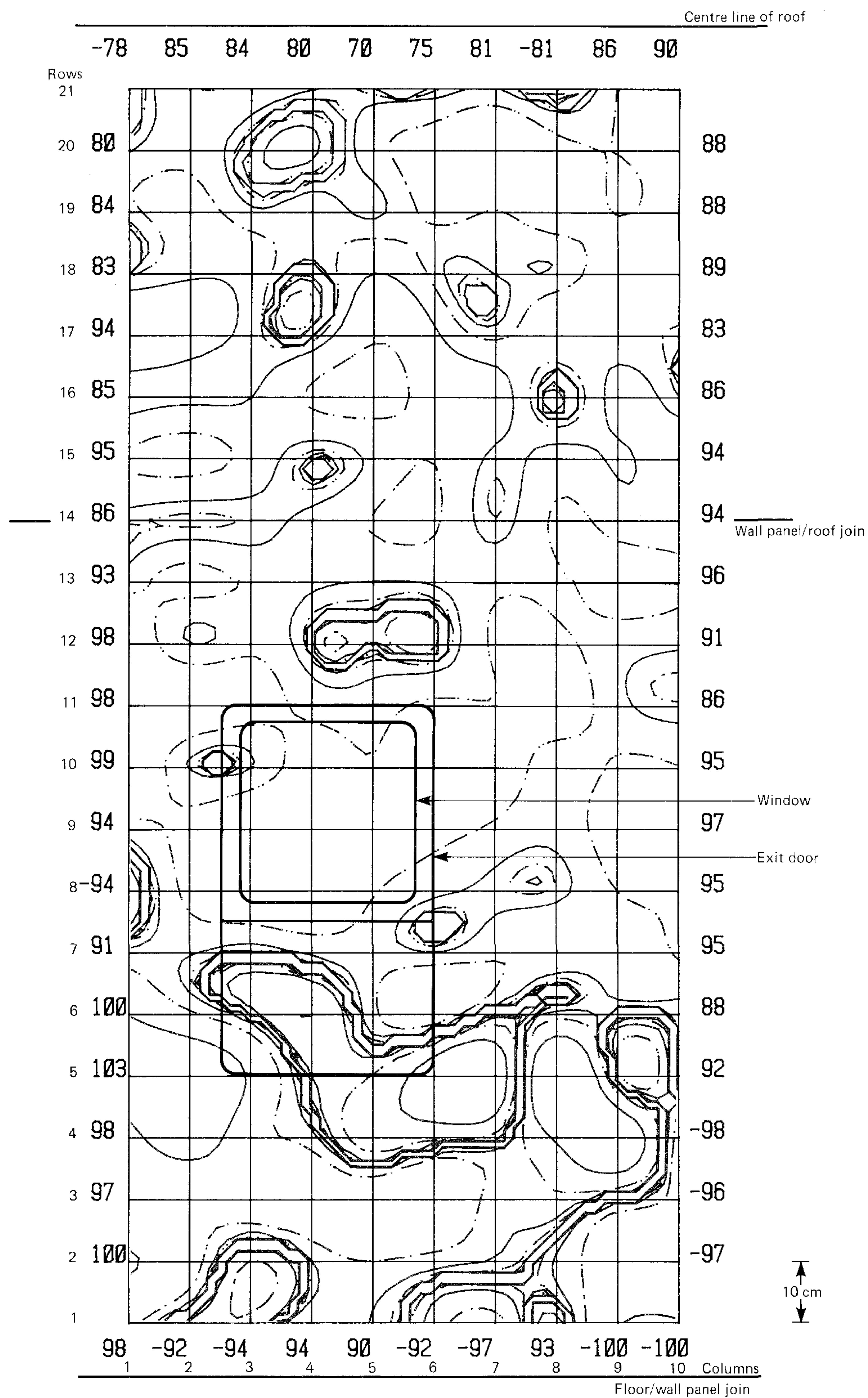
Fig. 17. Intensity map over the measurement surface for the 100Hz 1/3 octave band with 6 dB between the intensity contours. Linear interpolation with every second contour drawn dashed
